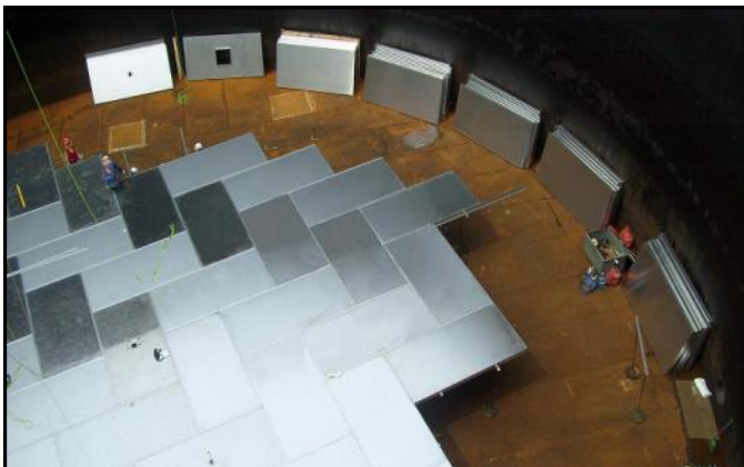
Sihanoukville, Cambodia IFR ID 34m x 6 Tanks, 2018
